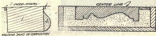
FIG. 57—SEE TEXT—FIG. 58—SECTION VIEW OF SIMPLE FLASK. SEE TEXT—SAND MOLDS
